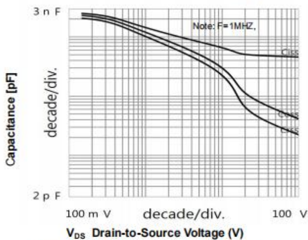
Figure 5.1 Capacitance Characteristics
