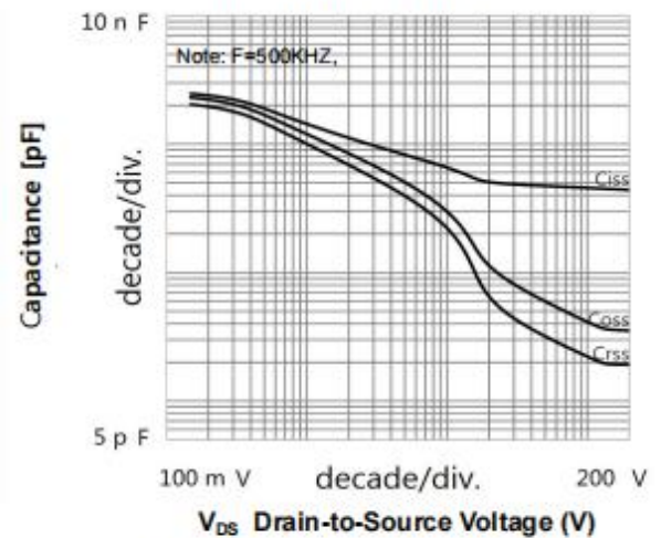
Figure 5.2 Capacitance Characteristics
