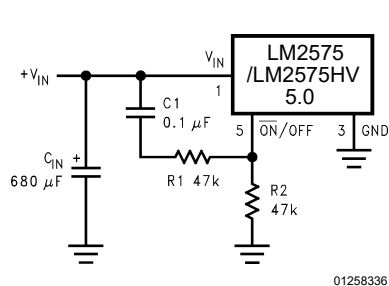
Figure 21. Delayed Startup
