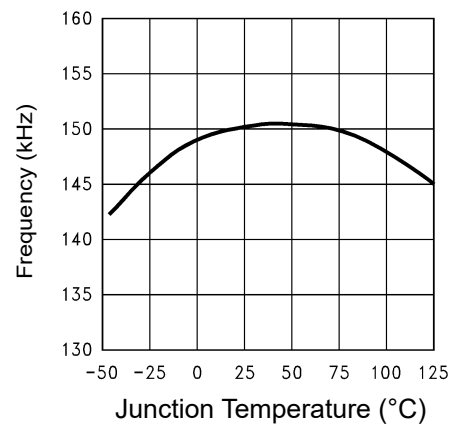
Figure 12: Switching Frequency
