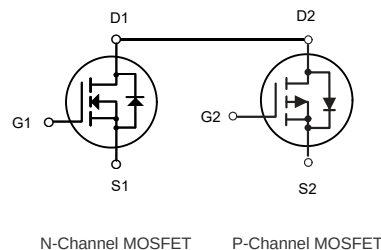
N-Channel MOSFET
