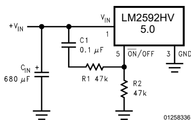
Figure 21. Delayed Startup
