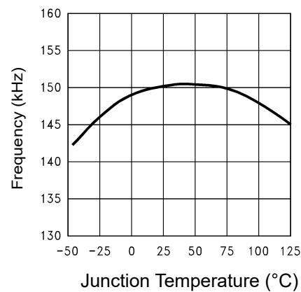
Figure 12: Switching Frequency
