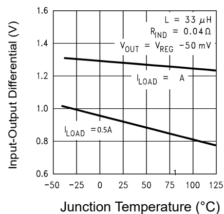
Figure 6: Dropout Voltage
