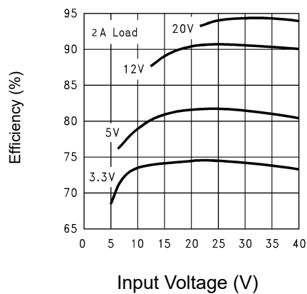
Figure 3: Efficiency
