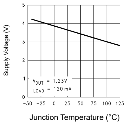
Figure 9: Supply Voltage
