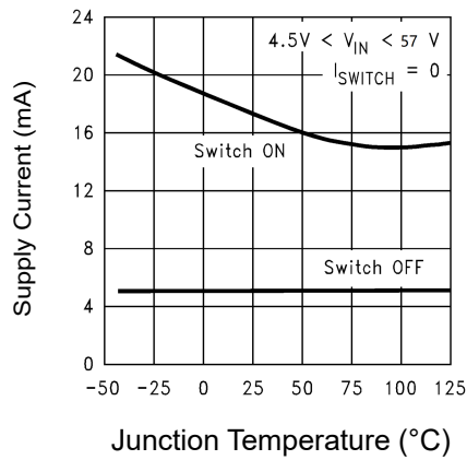
Figure 7: Quiescent Current
