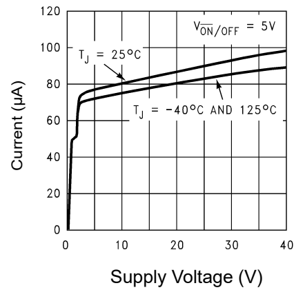
Figure 8: Quiescent Current
