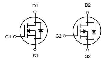
N-Channel
