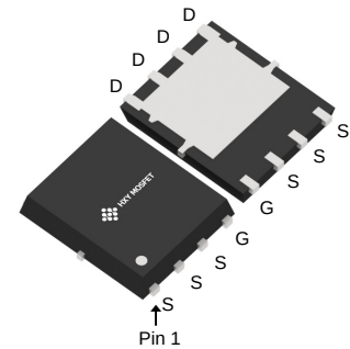
DFN5X6-8L (TDSO-8(5.9x5.2))
