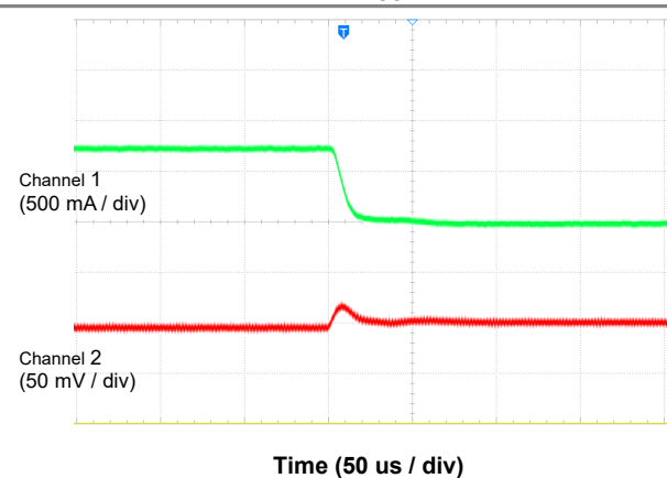
Channel 1 = I_{OUT} , channel 2 = V_{OUT} , V_{IN} = 1.8V, V_{OUT} = 0.8V Figure 18. Load Transient (750 mA to 1 mA)
