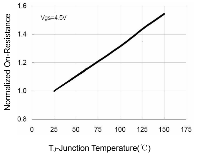
Figure 8 Drain-Source On-Resistance
