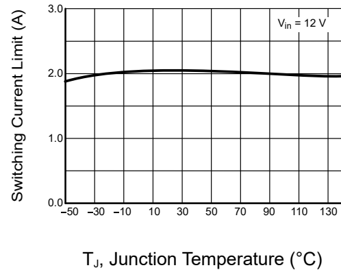
Figure 4: Current Limit
