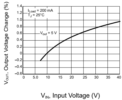
Figure 2: Line Regulation
