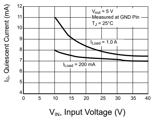
Figure 5: Quiescent Current
