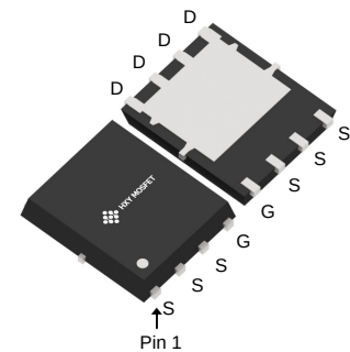
DFN5X6-8L (PQFN5x6)
