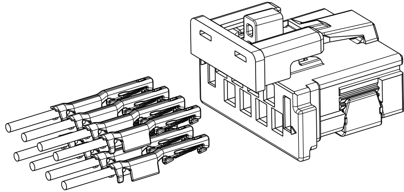
PRE-LOAD CONFIGURATION FOR TERMINAL INSERTION
