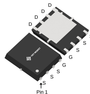
DFN5X6-8L (TDSON-8-EP(5x6))
