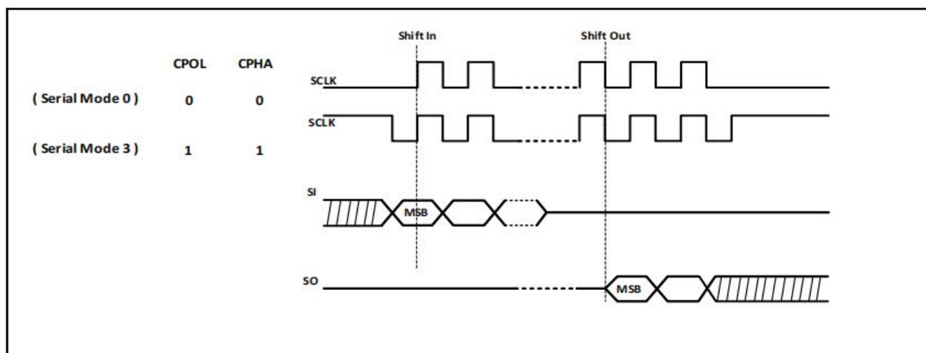
Figure-1. Serial Modes Supported (for Normal Serial Mode)
