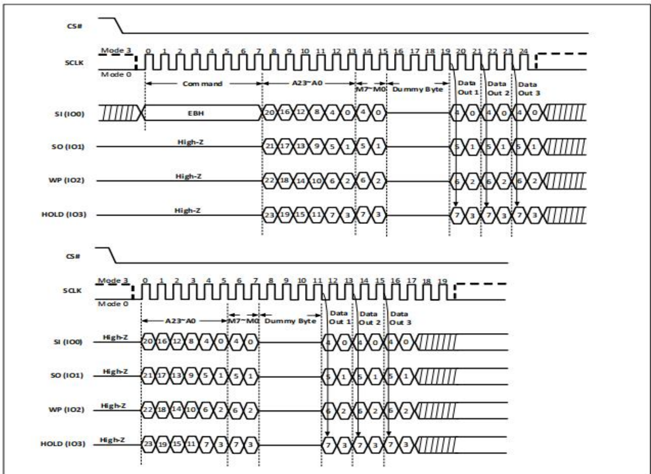
Figure-26. Quad I/O Fast Read with “Continuous Read Mode” Sequence Diagram (M5-4 = (1,0))
