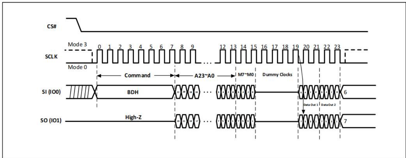
Figure-24. Quad Output Fast Read Sequence Diagram
