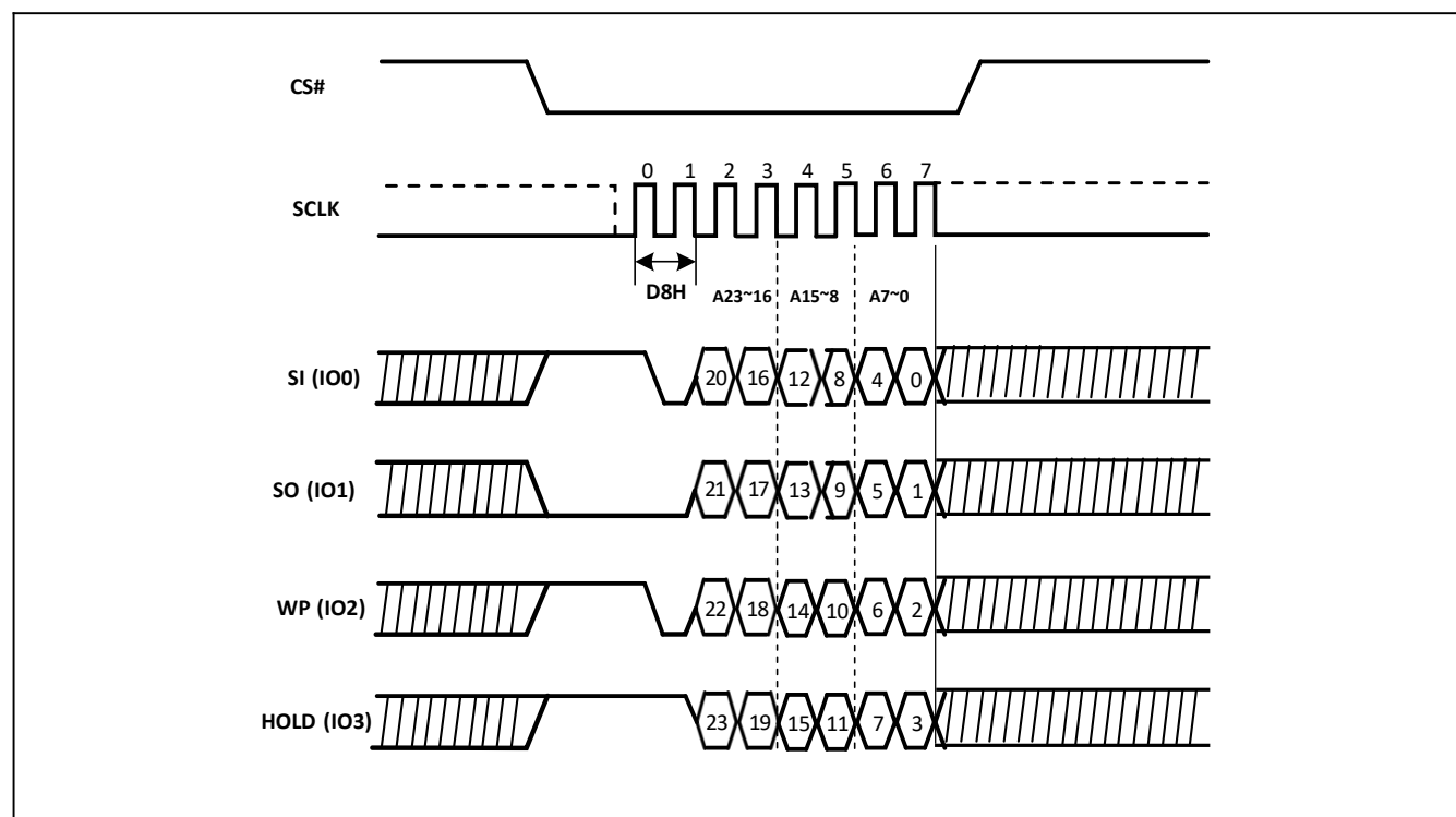
Figure-40. Block Erase Sequence Diagram (QPI)
