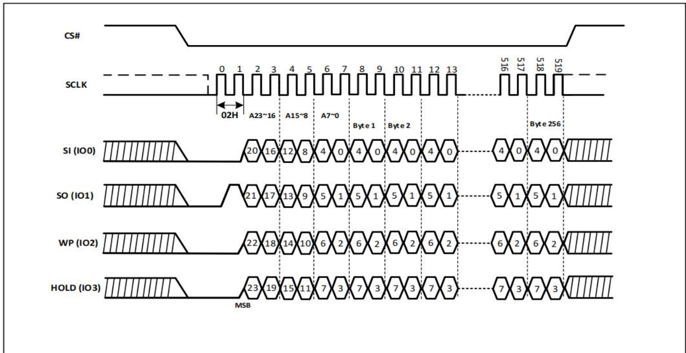
Figure-44. Page Program Sequence Diagram (QPI)
