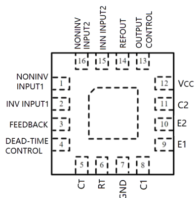
QFN-16 3*3
