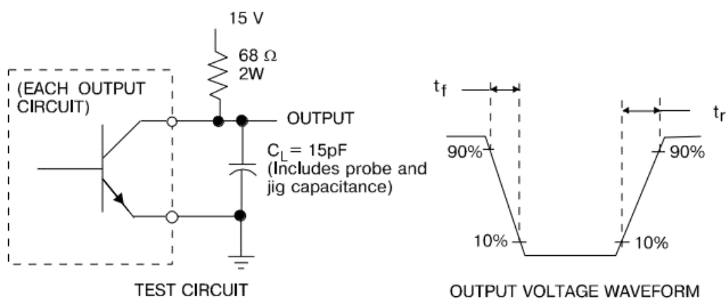
figure:2.amplifier characteristics
