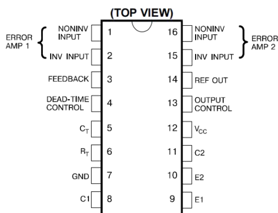
DIP/SOP/TSSOP/QSOP
