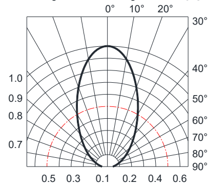
Fig.6-Radiation Diagram Ta=25°C
