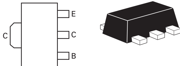
Pinout - top view
