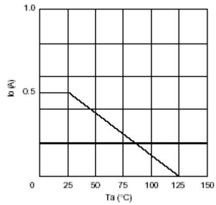
Fig.4 Derating curve
