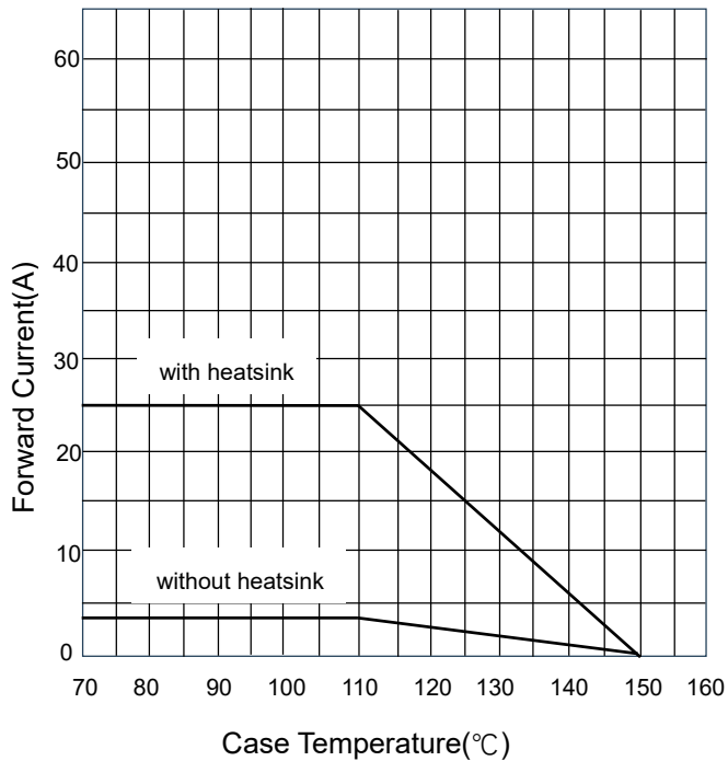
FIG 1: I_F - T_C
