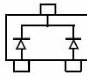
BAT54CT MARKING: L3
