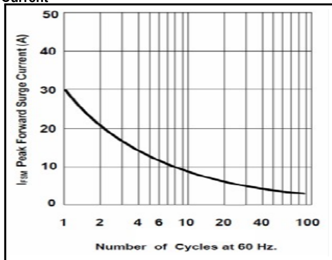
Figure 3: Maximum Non-Repetitive Peak Forward Surge
