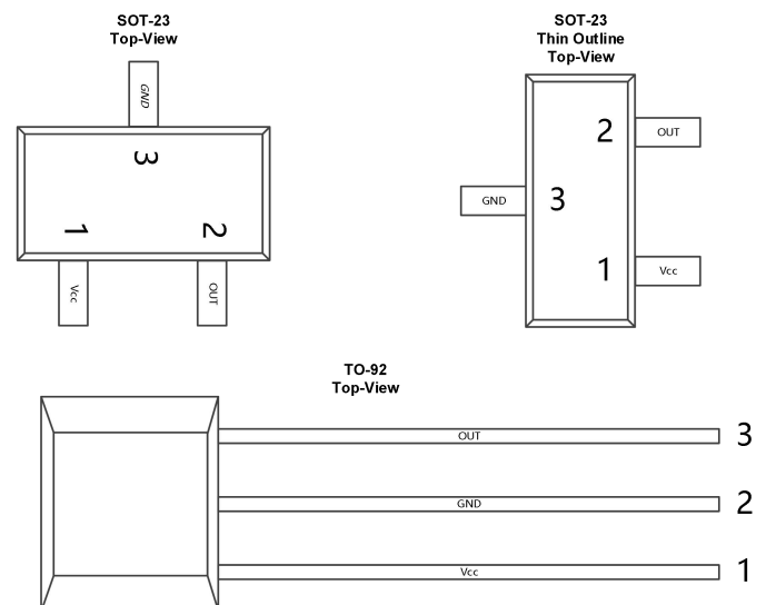
Figure.1 Pin Configuration & Functions
