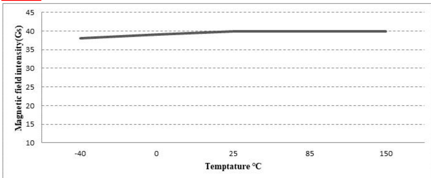
Figure.8 Magnetic Characteristics vs. Temperature (BHYS)
