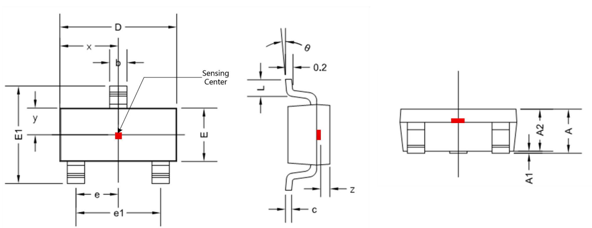
Figure.13 SOT-23 (Thin Outline) Package Drawing
