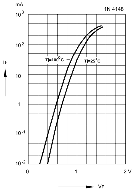
Forward characteristics
