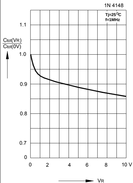
Relative capacitance versus reverse voltage
