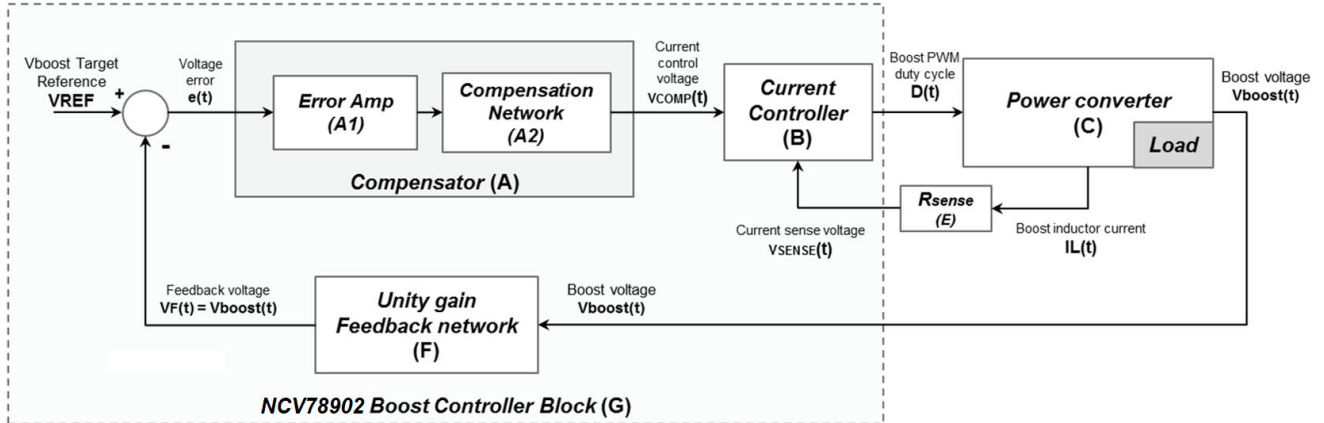
Figure 13. NCV78902 Boost Control Loop – Principle Block Diagram
