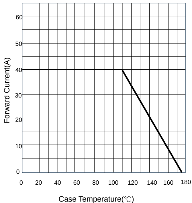
FIG 1: I_F - T_c
