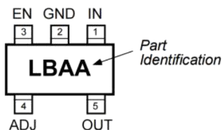
MIC5205-ADJ Adjustable Voltage
