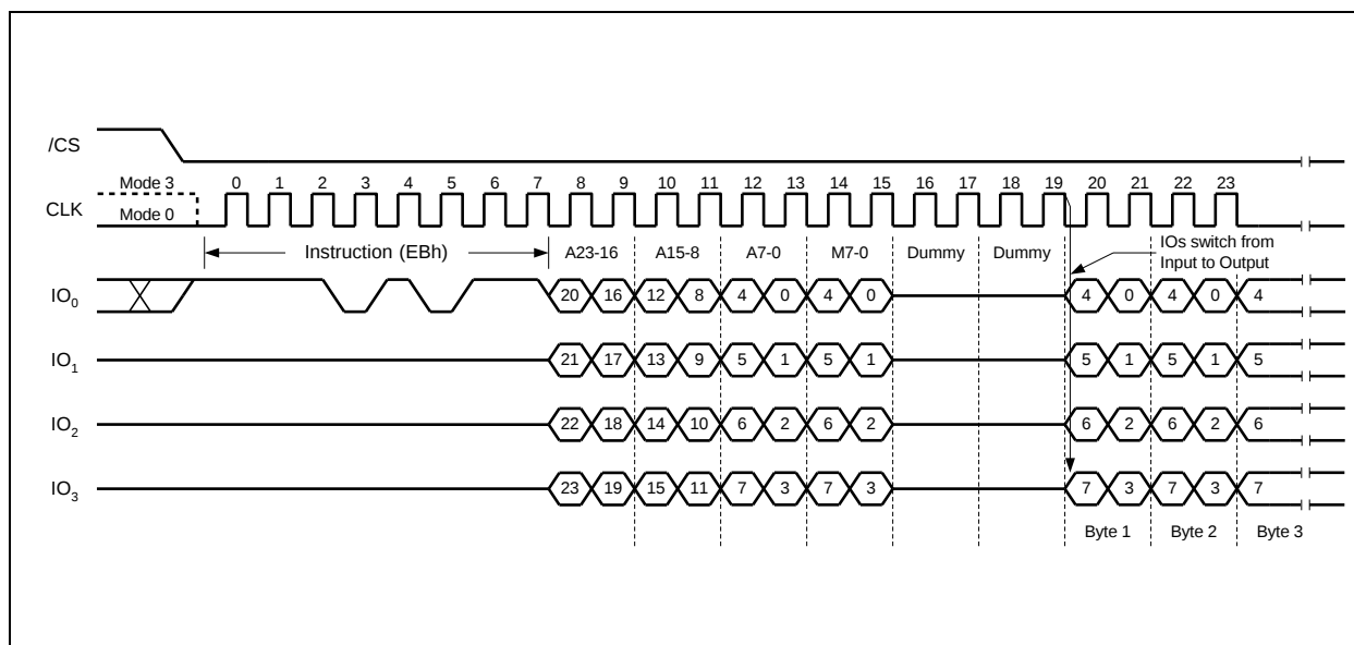
Figure 24. Fast Read Quad I/O (M7-M0 should be set to Fxh) 32-Bit Address is required when the device is operating in 4-Byte Address Mode
