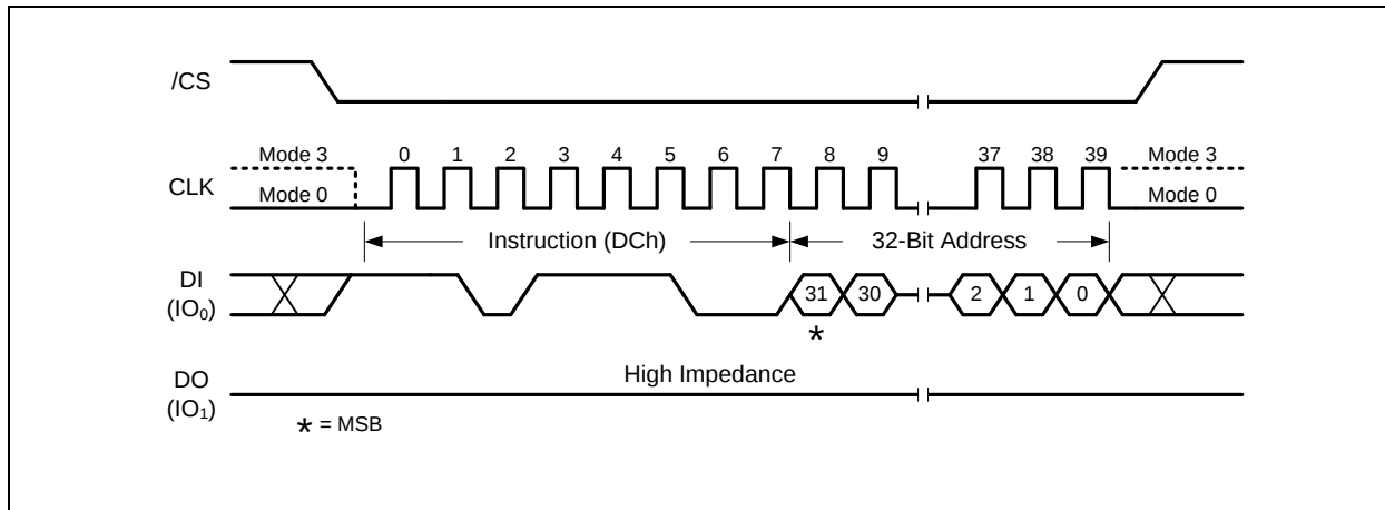
Figure 35. 64KB Block Erase with 4-Byte Address Instruction
