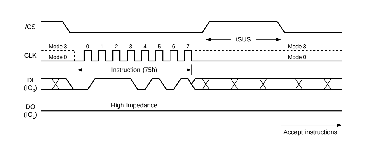
Figure 37. Erase/Program Suspend Instruction
