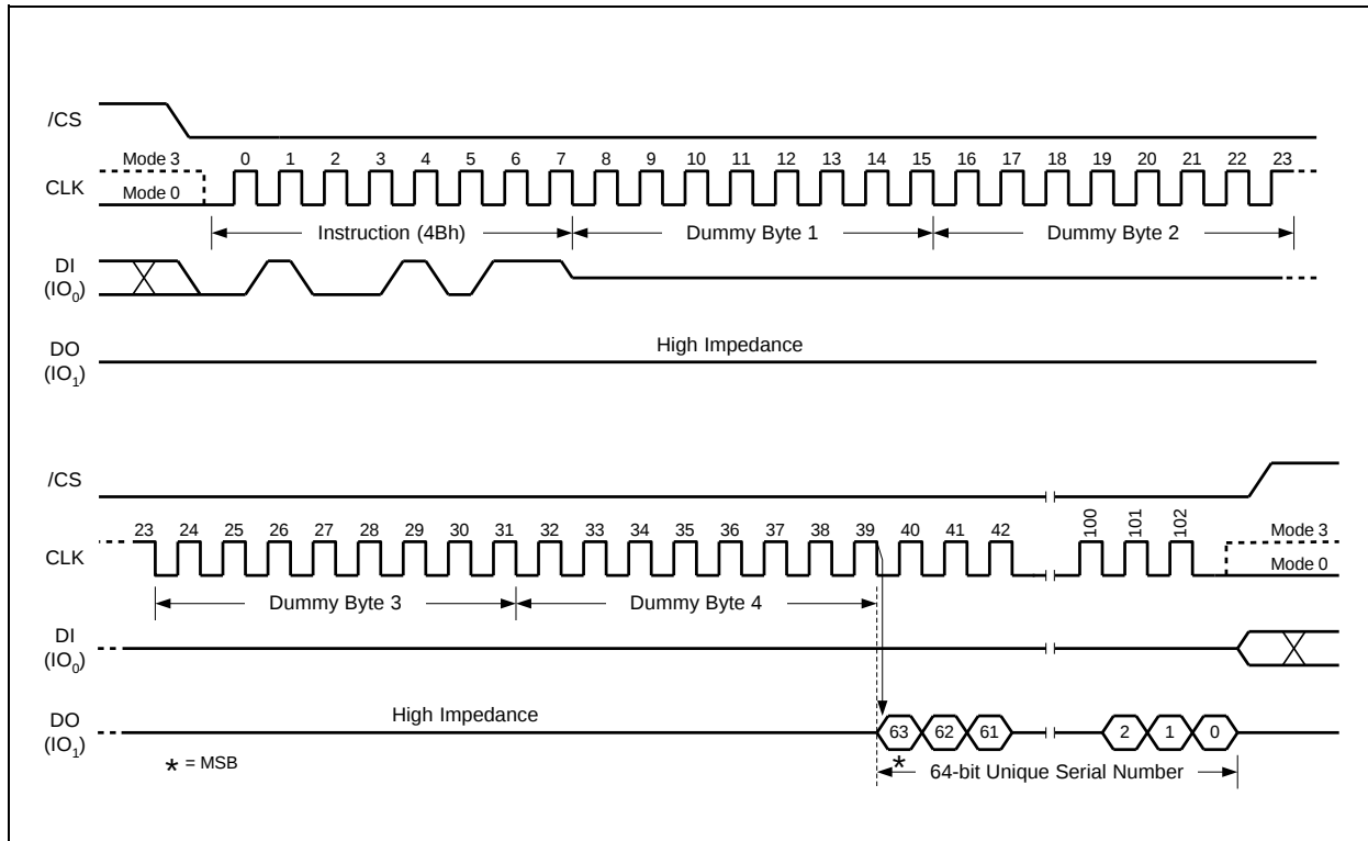
Figure 44. Read Unique ID Number Instruction 5 Dummy Bytes are required when the device is operating in 4-Byte Address Mode
