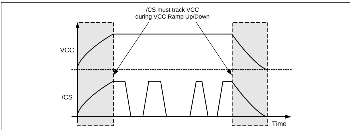
Figure 56b. Power-up, Power-Down Requirement
