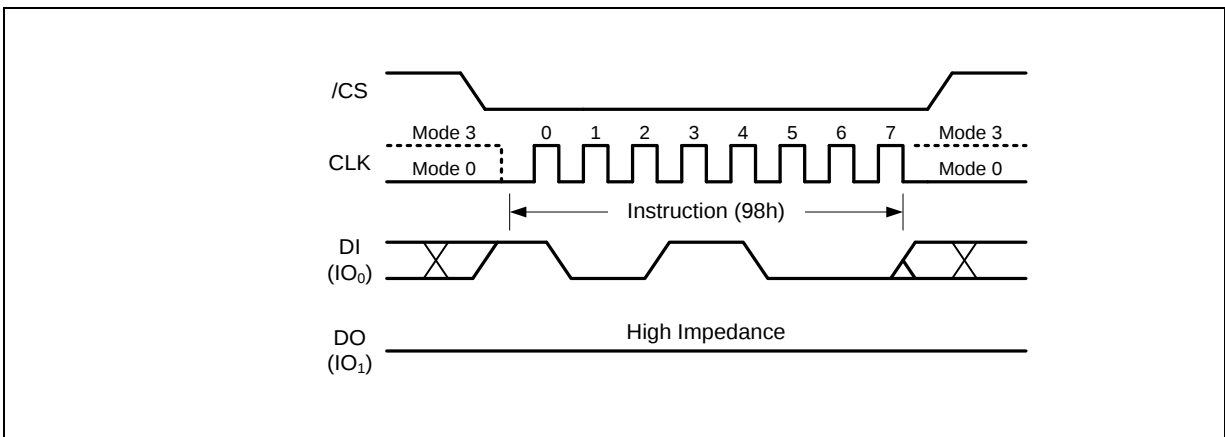
Figure 54. Global Block Unlock Instruction
