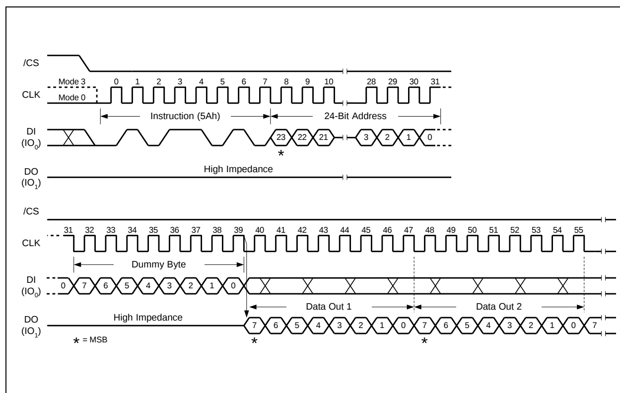
Figure 46. Read SFDP Register Instruction Sequence Diagram
