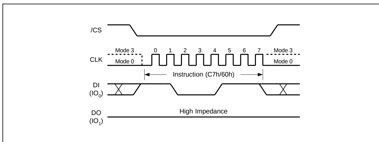
Figure 36. Chip Erase Instruction Sequence Diagram
