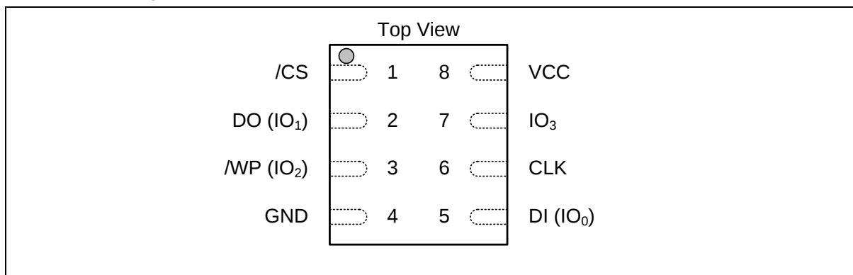
Figure 1a. W25Q256JV Pad Assignments, 8-pad WSON 8x6-mm (Package Code E)
