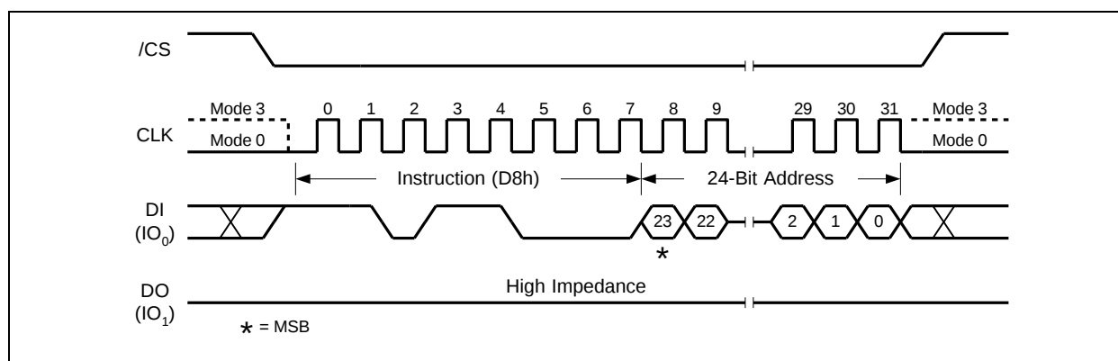
Figure 34. 64KB Block Erase Instruction
