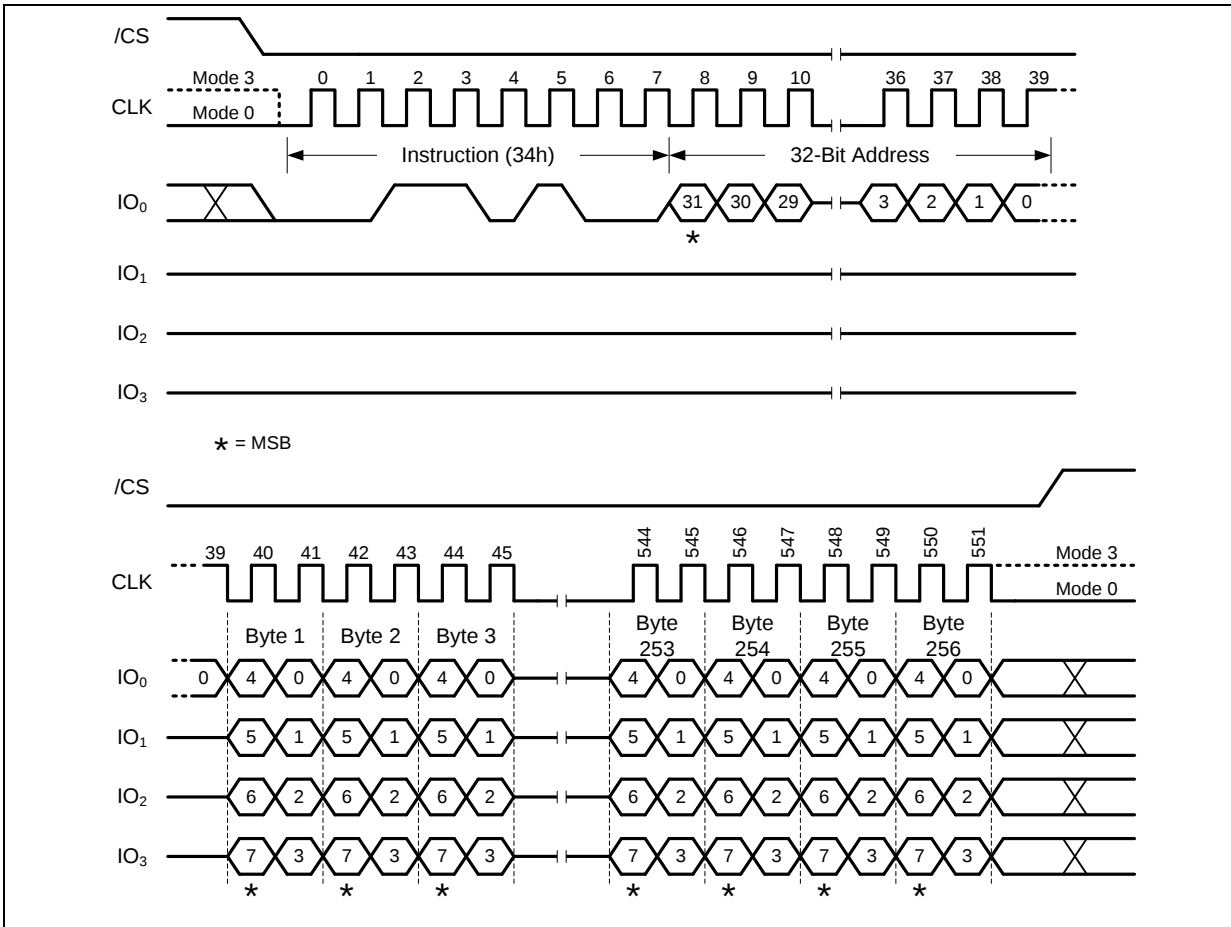
Figure 30. Quad Input Page Program with 4-Byte Addr.
