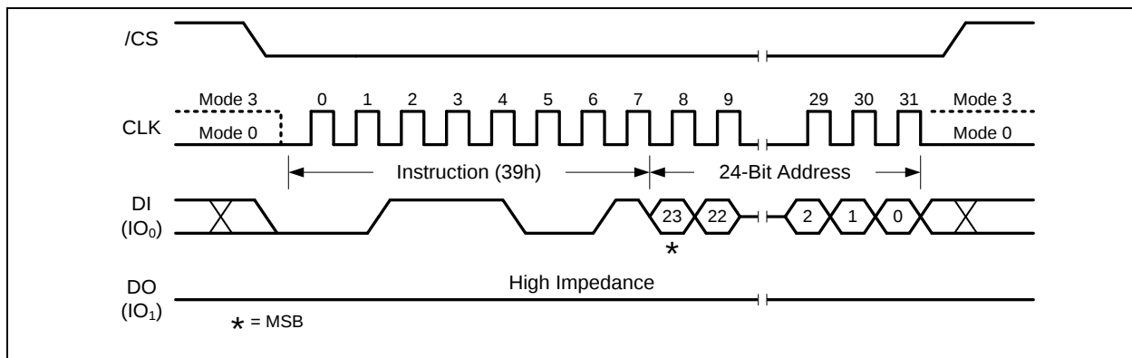
Figure 51. Individual Block Unlock Instruction 32-Bit Address is required when the device is operating in 4-Byte Address Mode
