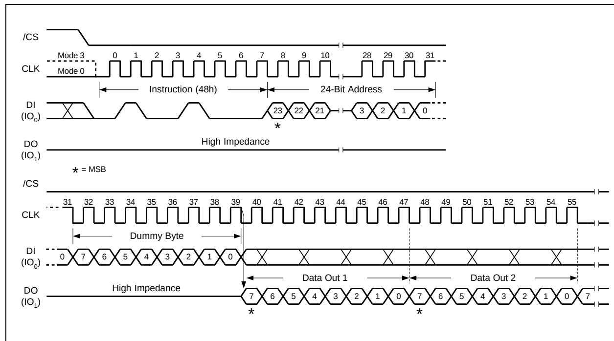
Figure 49. Read Security Registers Instruction 32-Bit Address is required when the device is operating in 4-Byte Address Mode
