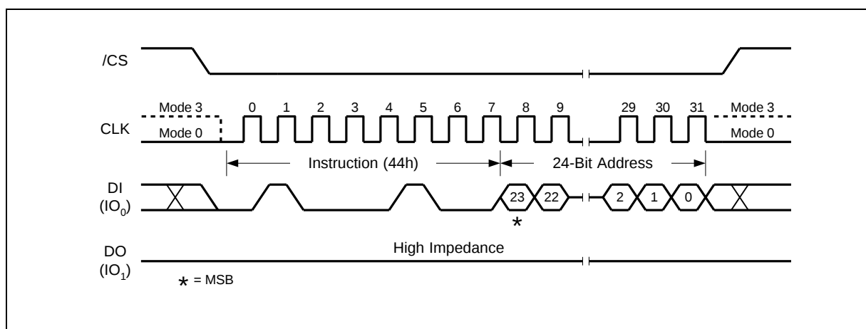
Figure 47. Erase Security Registers Instruction 32-Bit Address is required when the device is operating in 4-Byte Address Mode
