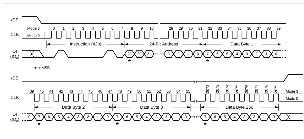
Figure 48. Program Security Registers Instruction 32-Bit Address is required when the device is operating in 4-Byte Address Mode
