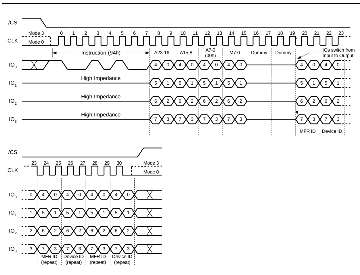
Figure 43. Read Manufacturer / Device ID Quad I/O Instruction 32-Bit Address is required when the device is operating in 4-Byte Address Mode
