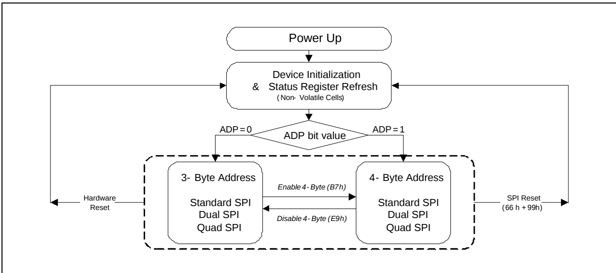
Figure 3. W25Q256JV Serial Flash Memory Operation Diagram
