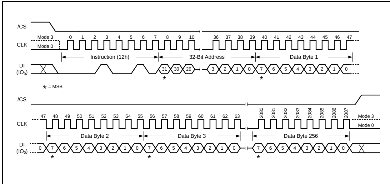
Figure 28. Page Program with 4-Byte Addr.
