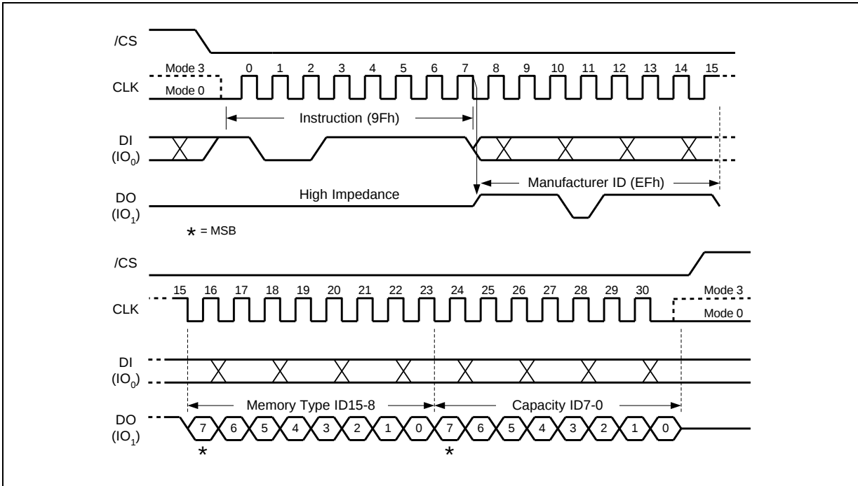
Figure 45. Read JEDEC ID Instruction
