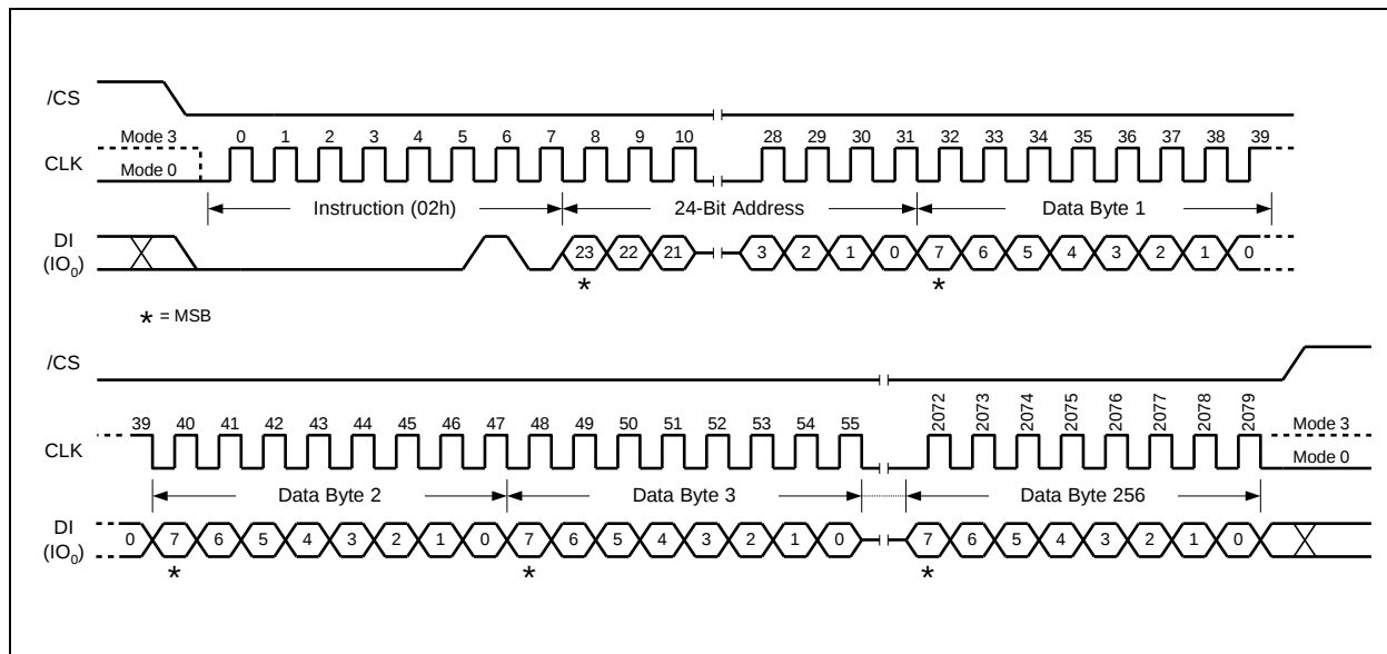
Figure 27. Page Program Instruction 32-Bit Address is required when the device is operating in 4-Byte Address Mode
