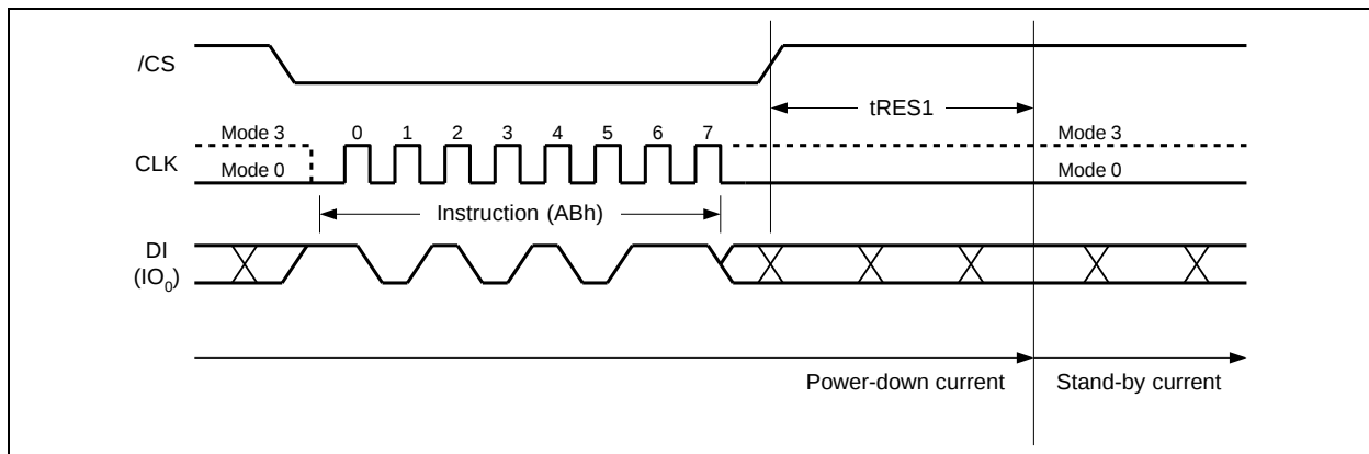
Figure 40a. Release Power-down Instruction
