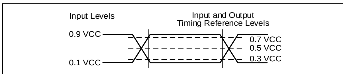
Figure 57. AC Measurement I/O Waveform
