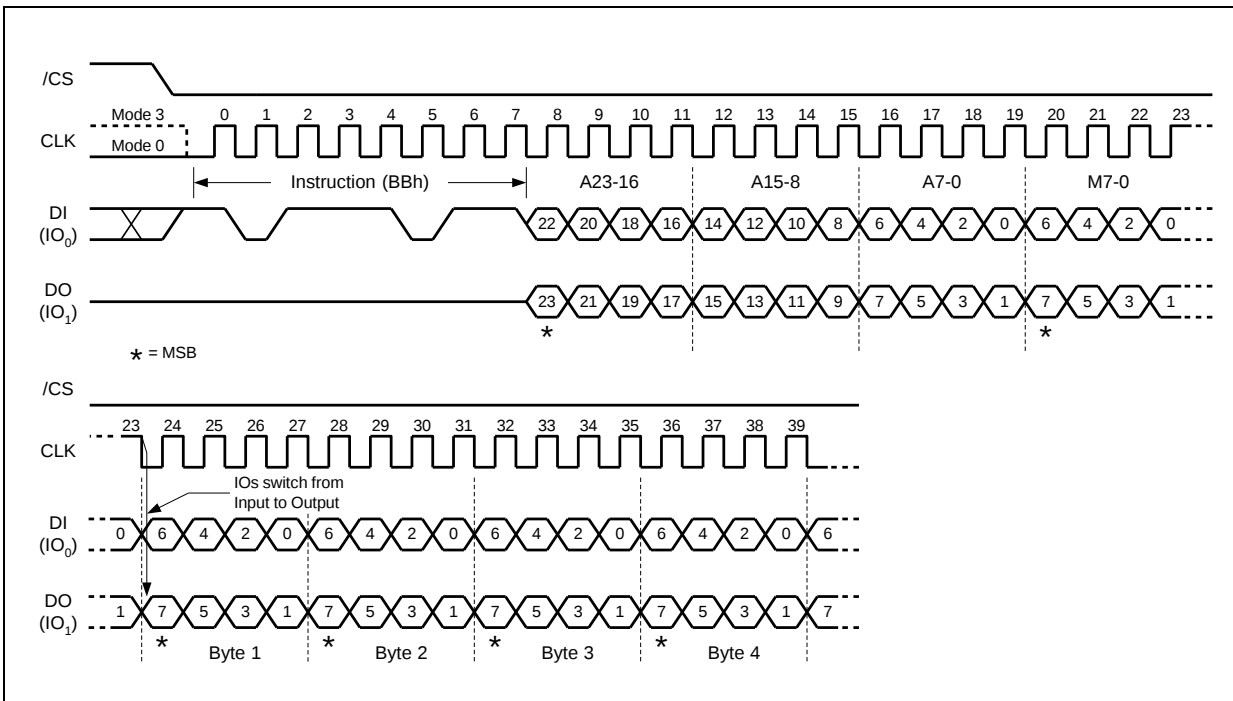
Figure 22. Fast Read Dual I/O (M7-M0 should be set to Fxh) 32-Bit Address is required when the device is operating in 4-Byte Address Mode
