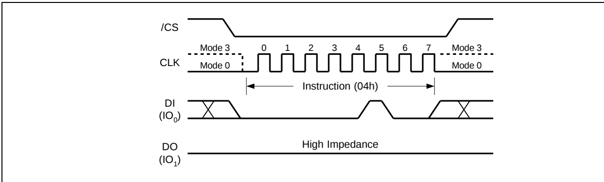
Figure 7. Write Disable Instruction for SPI Mode
