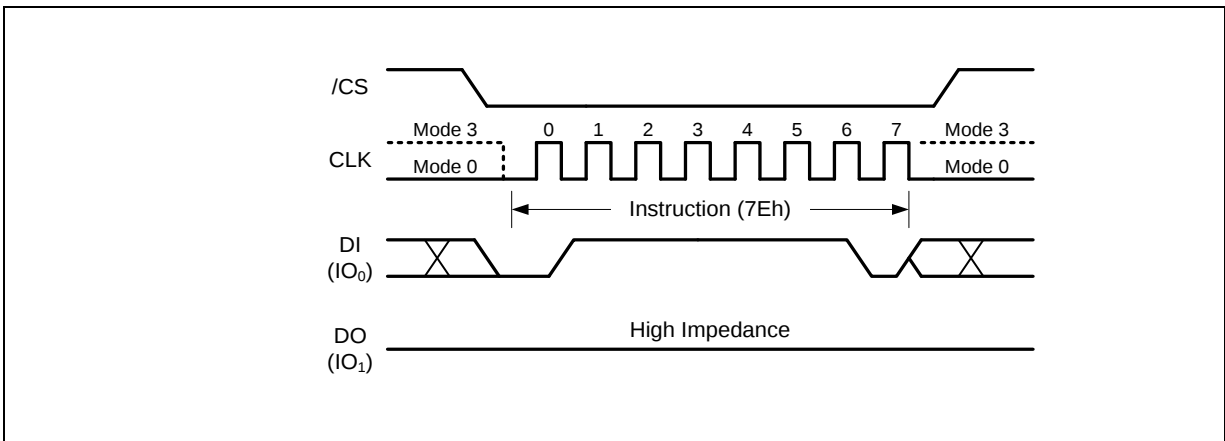
Figure 53. Global Block Lock Instruction for SPI
