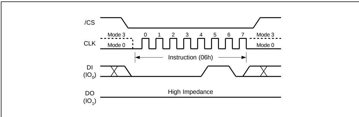
Figure 5. Write Enable Instruction
