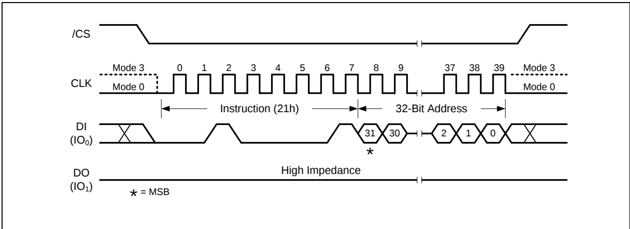
Figure 32. Sector Erase with 4-Byte Address Instruction
