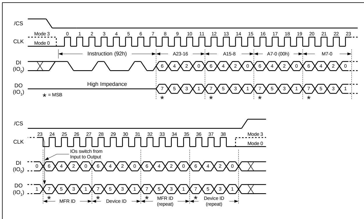
Figure 42. Read Manufacturer / Device ID Dual I/O Instruction 32-Bit Address is required when the device is operating in 4-Byte Address Mode
