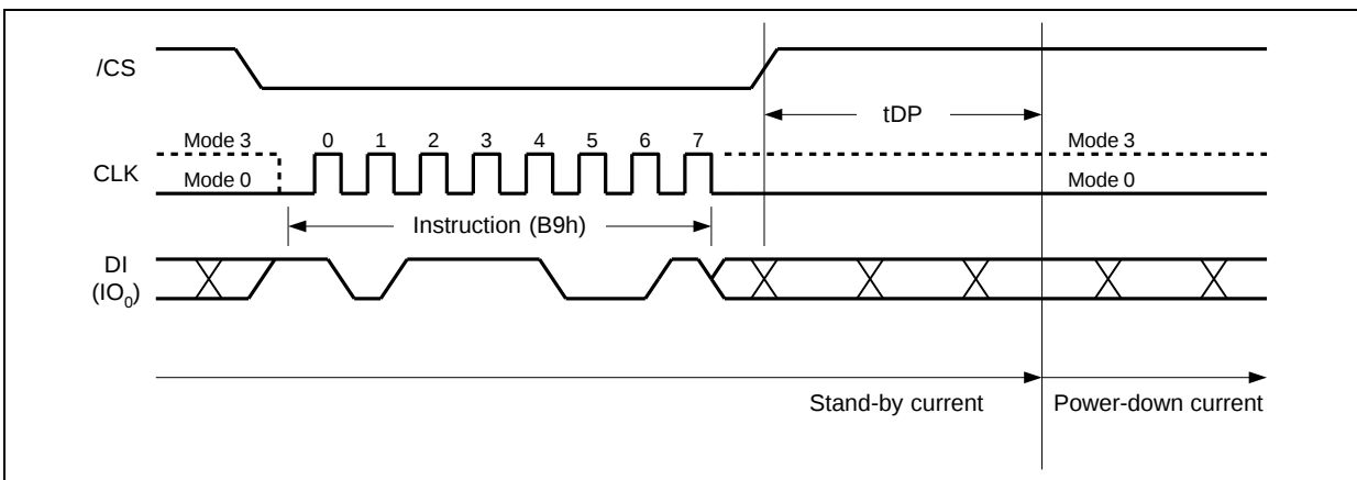
Figure 39. Deep Power-down Instruction
