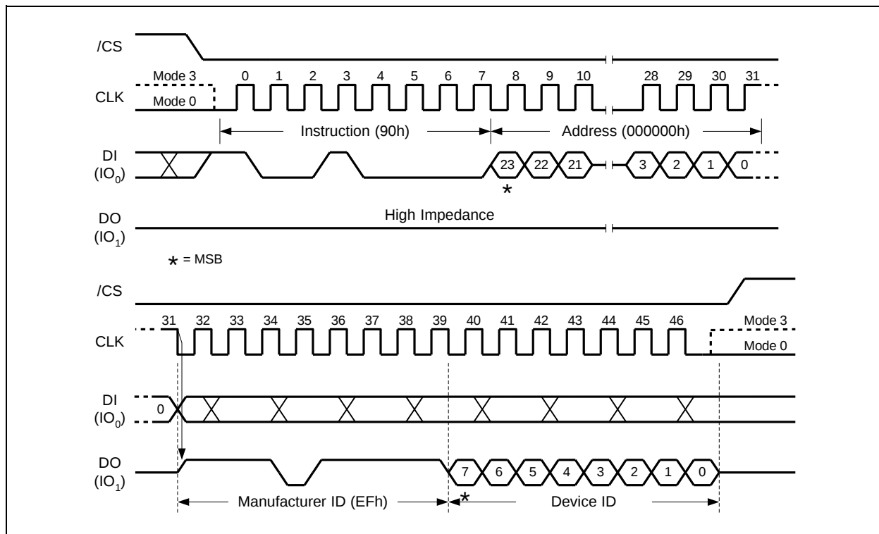
Figure 41. Read Manufacturer / Device ID Instruction
