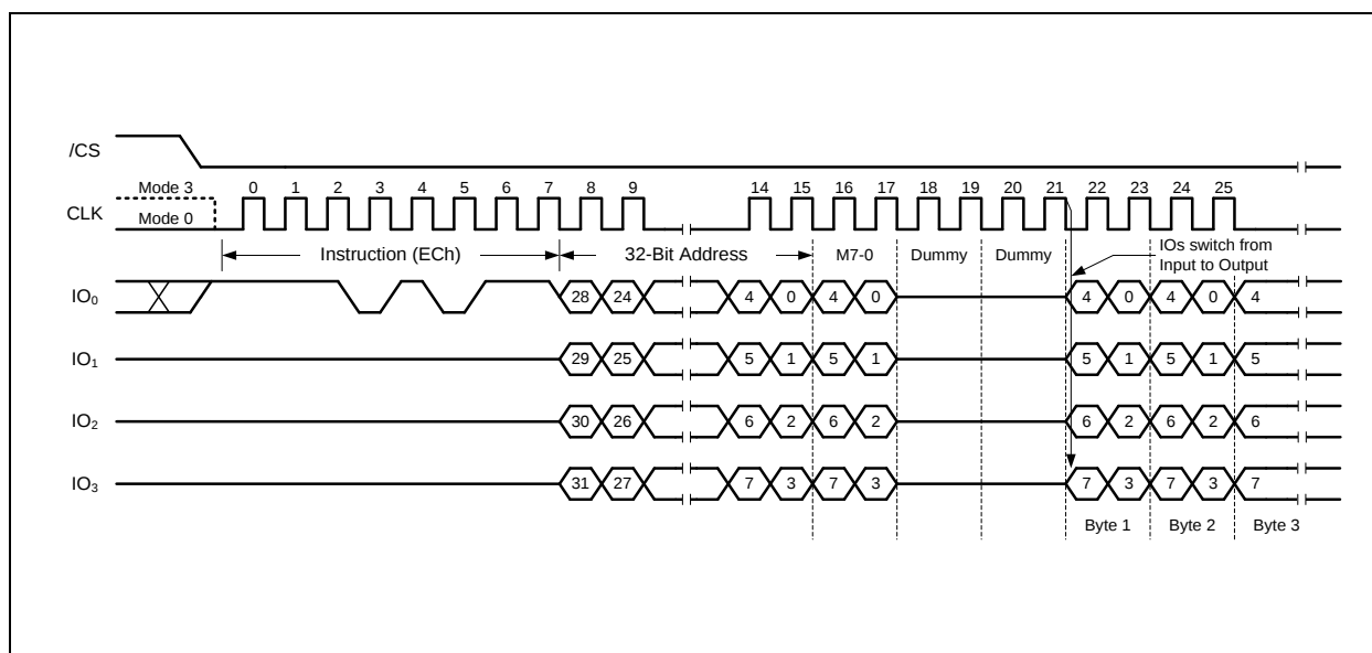
Figure 25. Fast Read Quad I/O w/ 4-Byte Addr. (M7-M0 should be set to Fxh)
