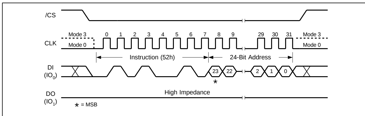
Figure 33. 32KB Block Erase Instruction
