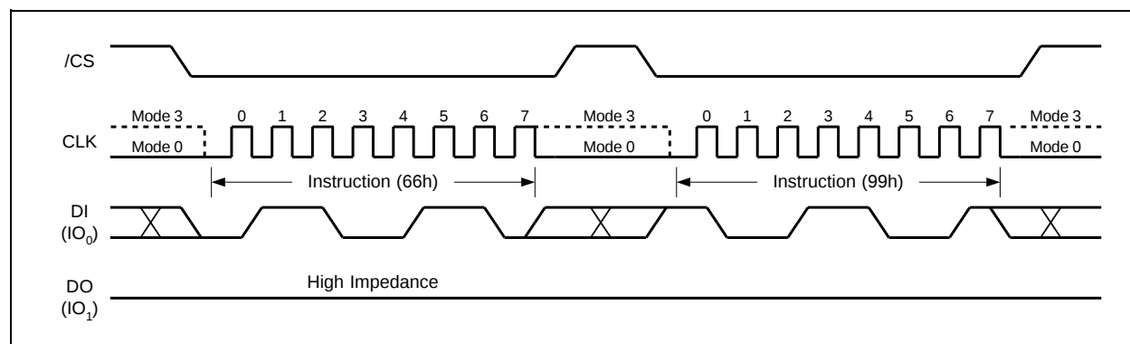
Figure 55. Enable Reset and Reset Instruction Sequence
