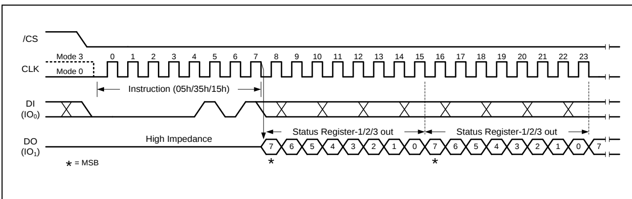
Figure 8. Read Status Register Instruction
