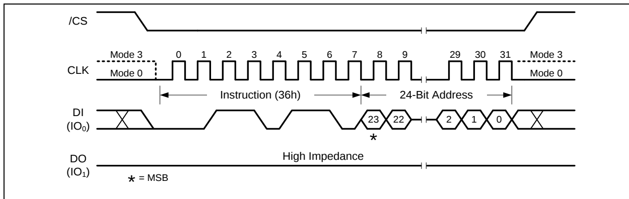
Figure 50. Individual Block/Sector Lock Instruction 32-Bit Address is required when the device is operating in 4-Byte Address Mode
