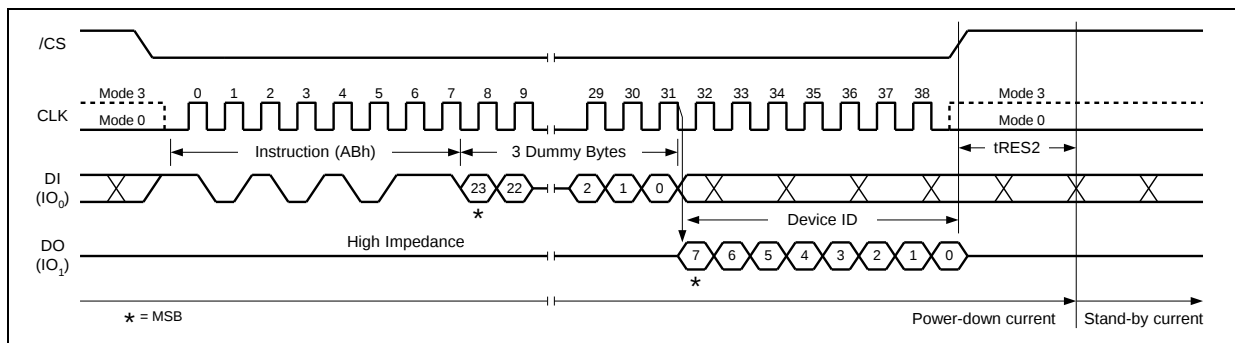
Figure 40b. Release Power-down / Device ID Instruction
