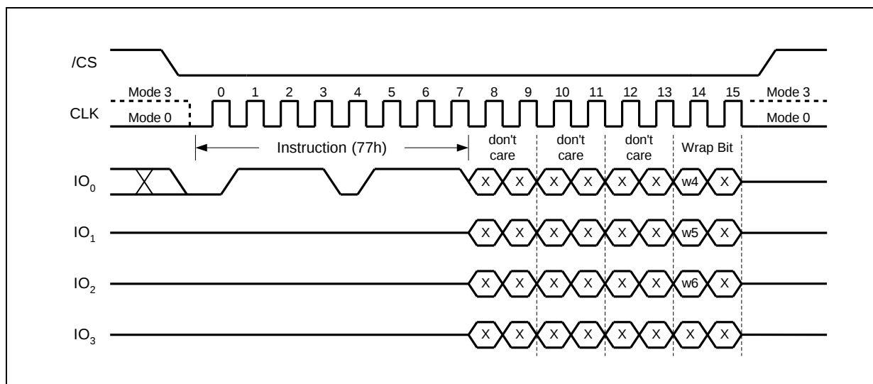
Figure 26. Set Burst with Wrap Instruction
