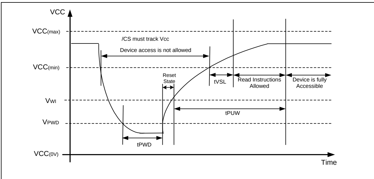
Figure 56a. Power-up Timing and Voltage Levels
