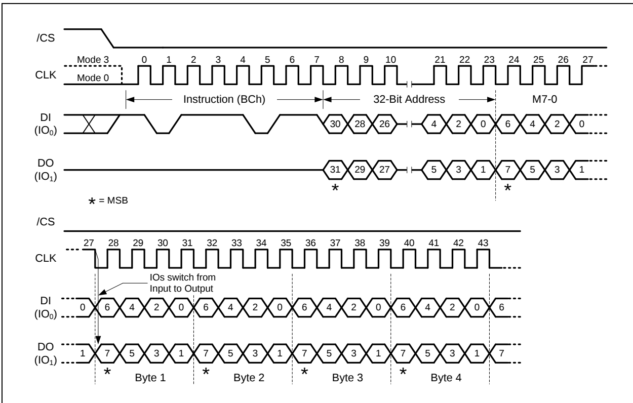
Figure 23. Fast Read Dual I/O w/ 4-Byte Addr. (M7-M0 should set to Fxh, SPI Mode only)
