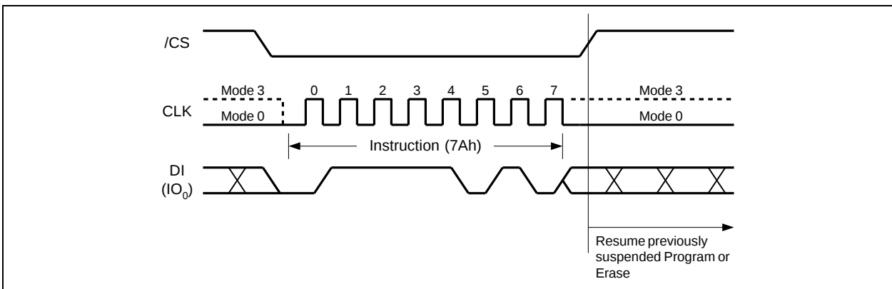
Figure 38. Erase/Program Resume Instruction
