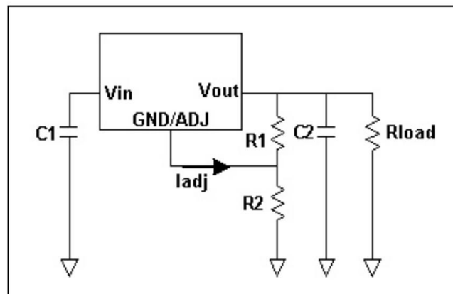
Figure 2 AT1117 Adjustable Application Circuit
