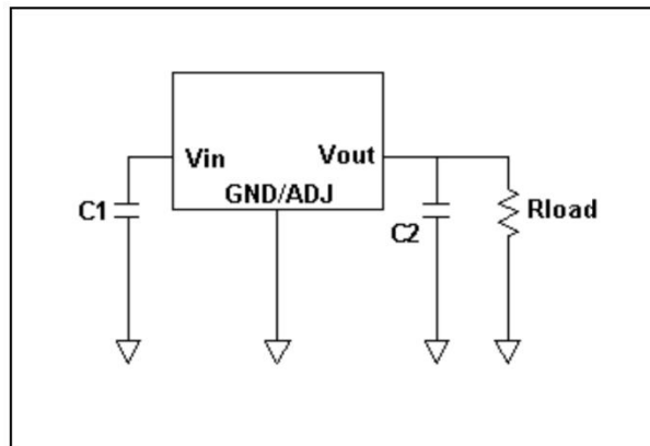
Figure 1 AT1117 Fixed Voltage Version Application Circuit
