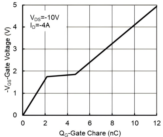
Figure 6: Gate-Charge Characteristics
