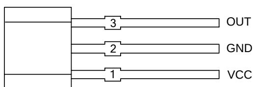
Figure 1. Pin Configuration of SL49 E (Front View)
