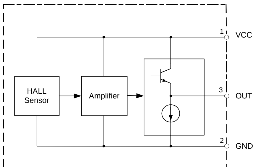
Figure 2. Functional Block Diagram of SL49E
