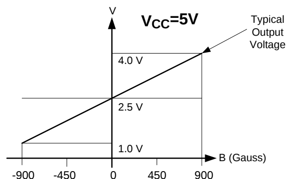
Figure 3. The Transfer Characteristics of SL49E
