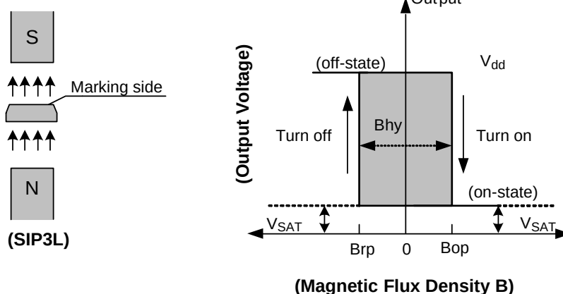
Figure 5. Operating Characteristics of SL177
