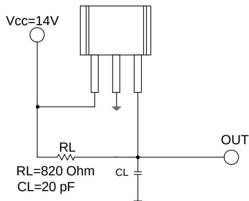
Figure 4. Test Circuit
