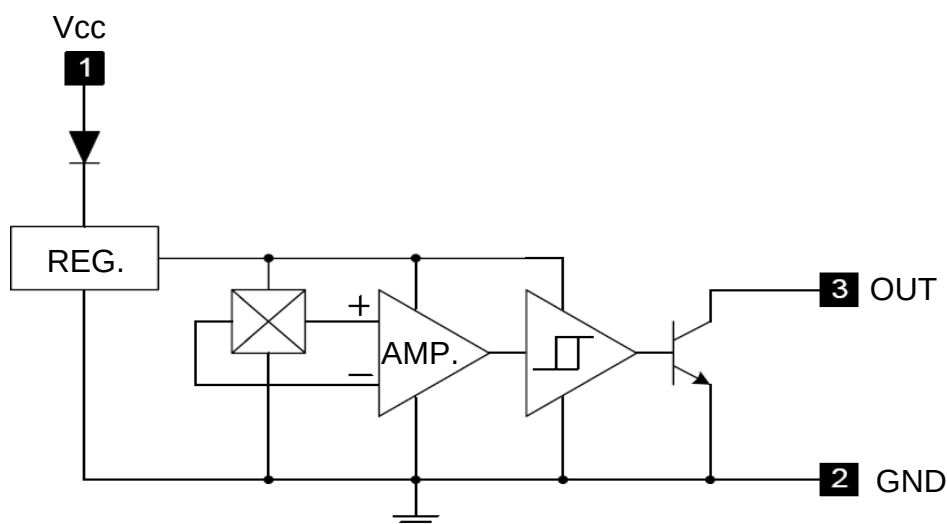
Figure 3. Function Block Diagram of SL177
