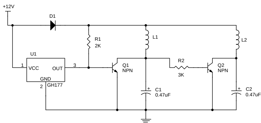
Figure 1. Typical Application of SL177 in Brush-less DC Fan.
