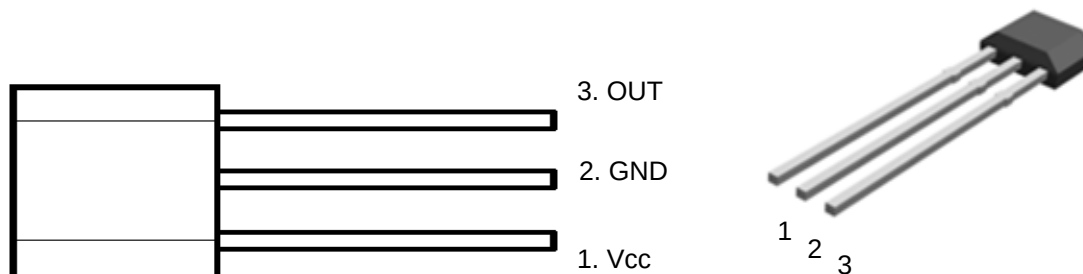
Figure 2. Pin Configuration of SL177 (Front View)
