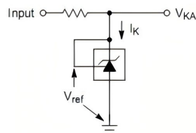
Test Circuit for V_{KA} = V_{ref}
