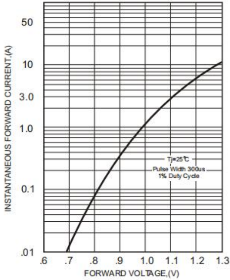
FIG.1-TYPICAL FORWARD CHARACTERISTICS
