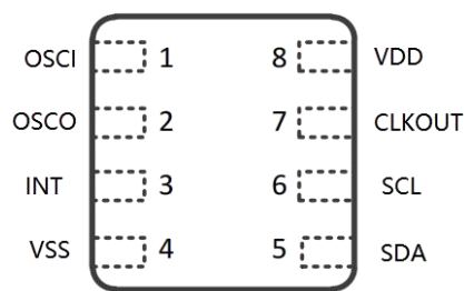
DFN-8 3*3
