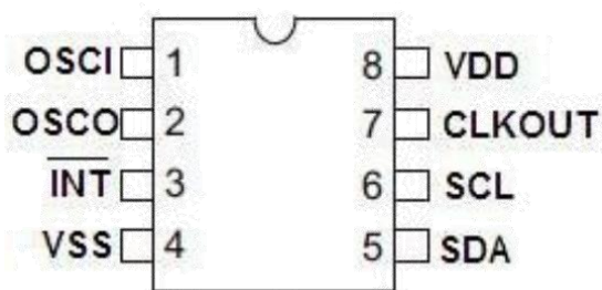
SOP-8/MSOP-8/DIP-8
