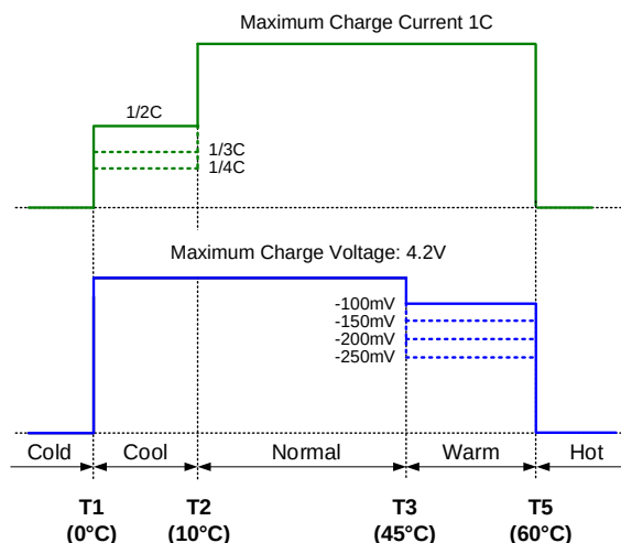
Figure 7: NTC JEITA Profile
