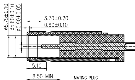
MATING PLUG
