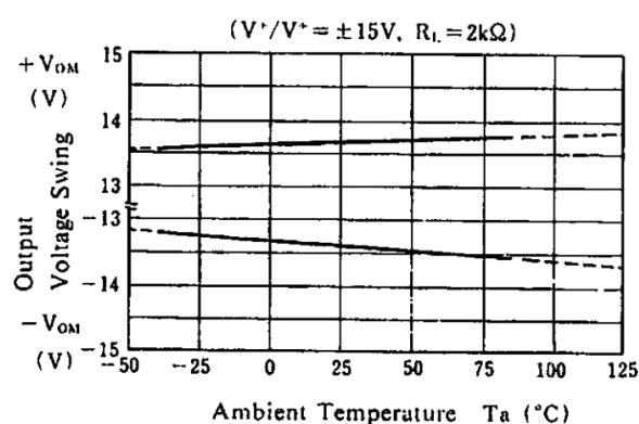
Output Voltage Swing vs. Temperature
