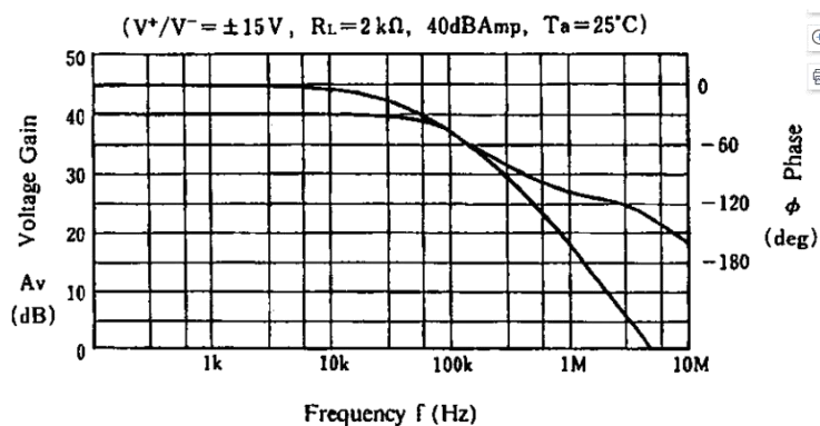
Voltage Gain, Phase vs. Frequency
