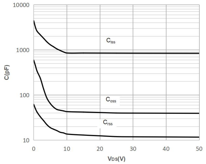
Figure 6: Capacitance Characteristics
