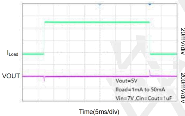
Load-Transient Response
