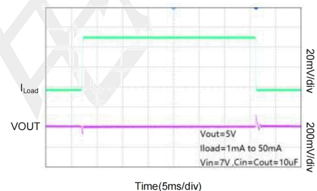
Load-Transient Response
