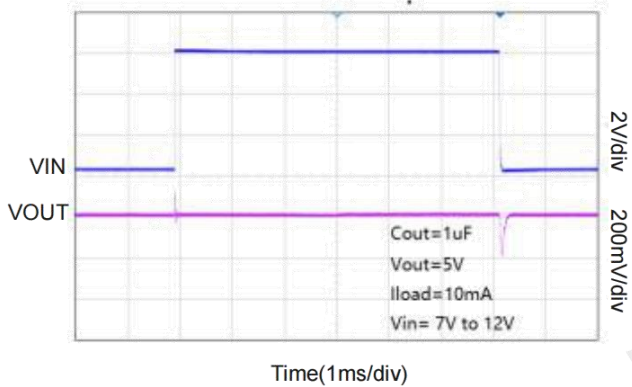
Line-Transient Response
