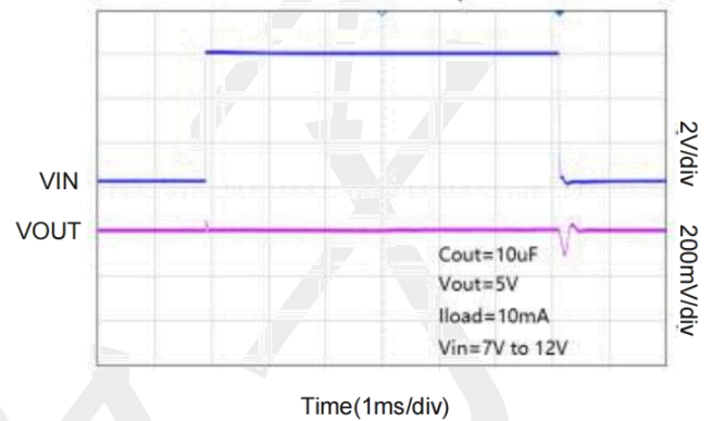
Line-Transient Response
