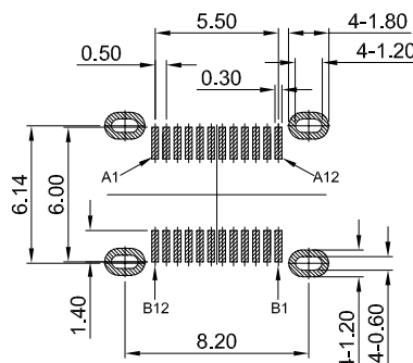
PCB REFERENCE DIAGRAM TOLERANCE:±0.05
