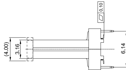
WITHOUT CAP
