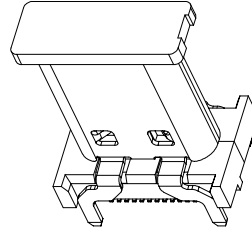
WITH CAP
