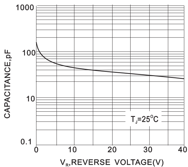
FIG. 3-TYPICAL JUNCTION CHATACTERISTIC
