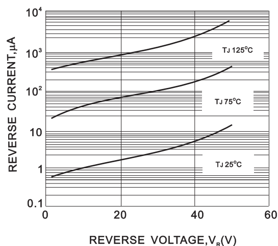
FIG. 2-TYPICAL REVERSE CHARACTERISTIC
