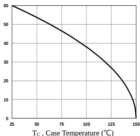
Fig.2 Continuous Drain Current vs. T_c
