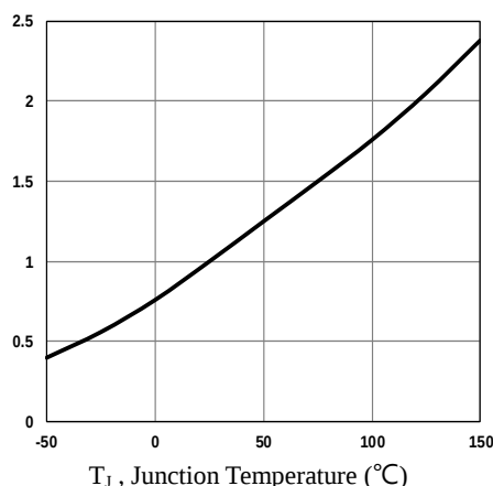
Fig.3 Normalized R_{DS(on)} vs. T_j
