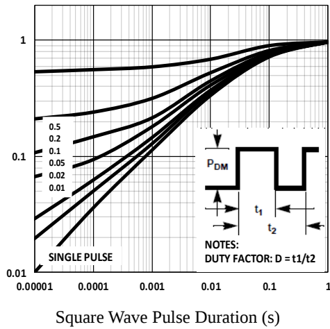
Fig.9 Normalized Transient Impedance
