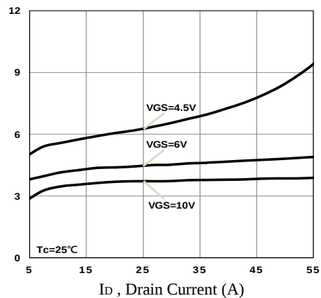
Fig.6 Turn-On Resistance vs. I_D
