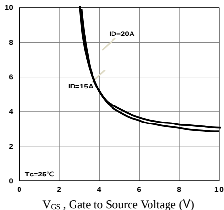
Fig.5 Turn-On Resistance vs. V_{GS}
