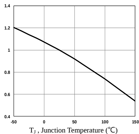
Fig.4 Normalized V_{th} vs. T_j
