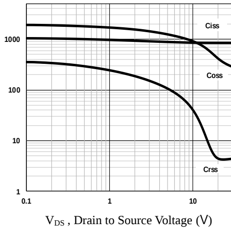
Fig.7 Capacitance Characteristics
