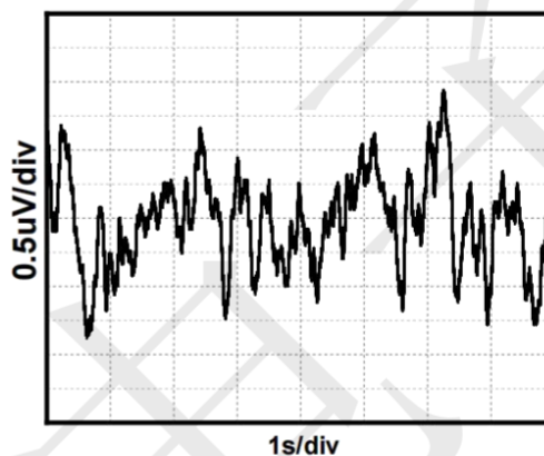
Figure 3. 0.1Hz to 10Hz Noise
