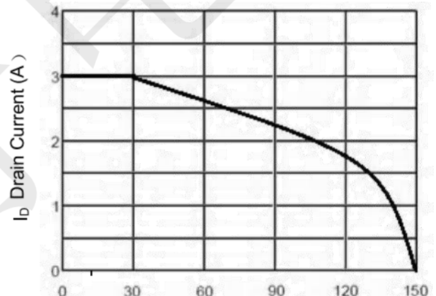
Figure 4 Drain Current
