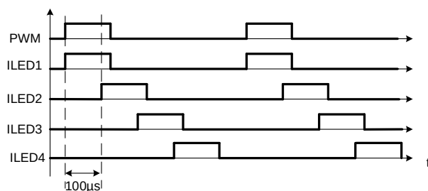
Figure 6: 100 \mu s Delay Time with 4 Channels
