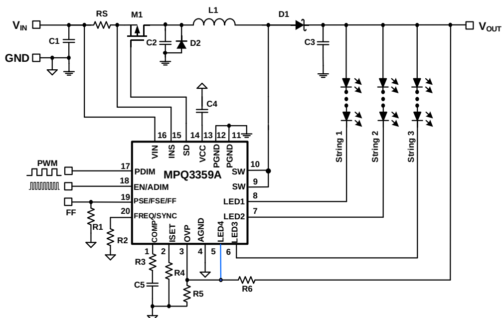
Figure 2: Typical Application with 3 Strings (Connect LED4 to the OVP Pin)
