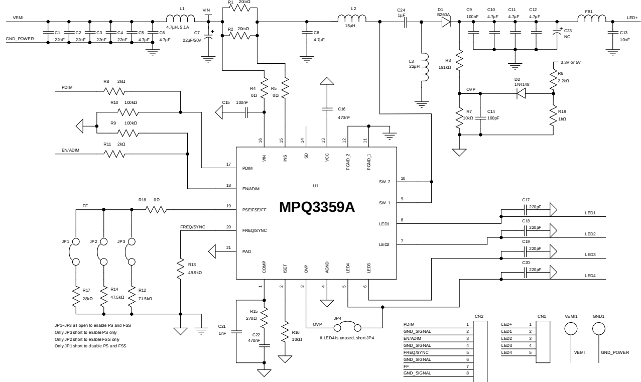
Figure 10: Typical Application Circuit (SEPIC)
