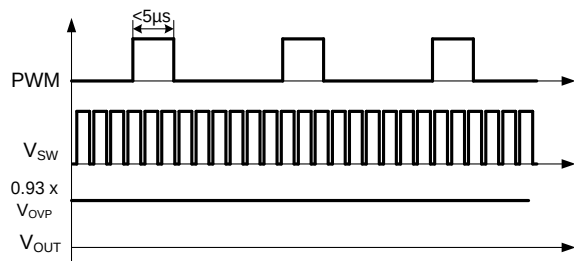
Figure 4: Deep Dimming Ratio for PWM Dimming
