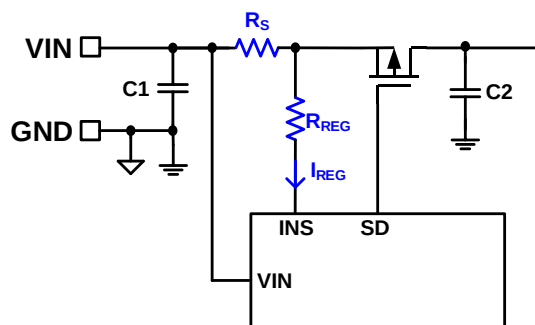
Figure 7: Typical VIN Current Detection Circuit
