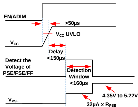
Figure 5: PSE/FSE/FF Pin Timing
