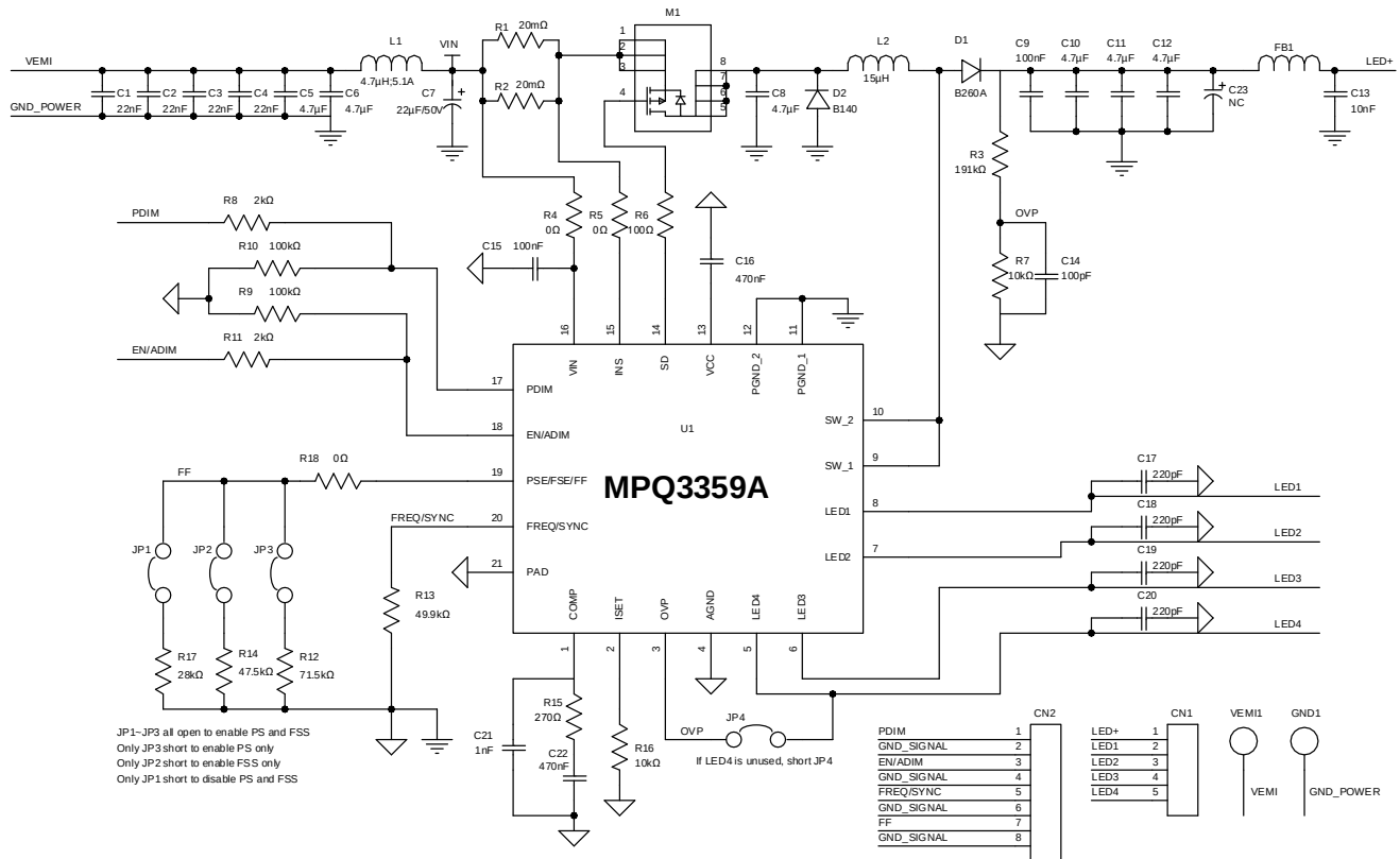
Figure 9: Typical Application Circuit (Boost)
