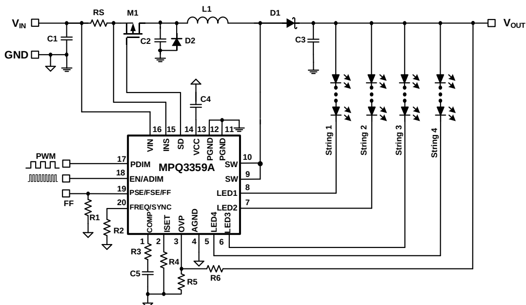
Figure 1: Typical Application with 4 Strings
