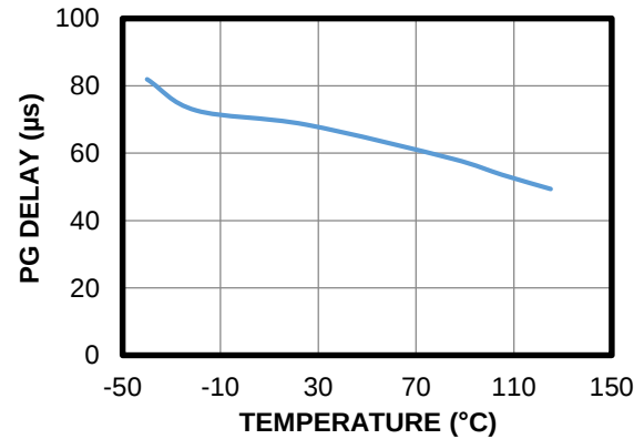
PG Delay vs. Temperature
