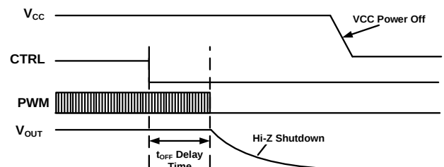
Figure 10: Shutdown Sequence with Hi-Z Shutdown
