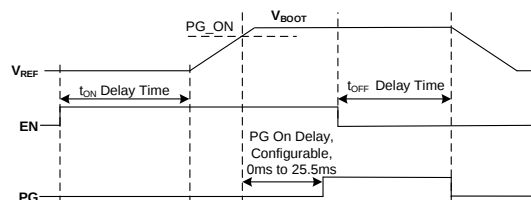
Figure 17: Power Good On/Off Sequence
