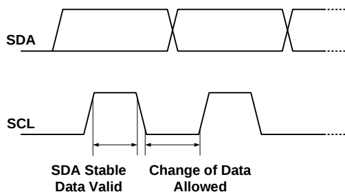
Figure 9: Bit Transfer
