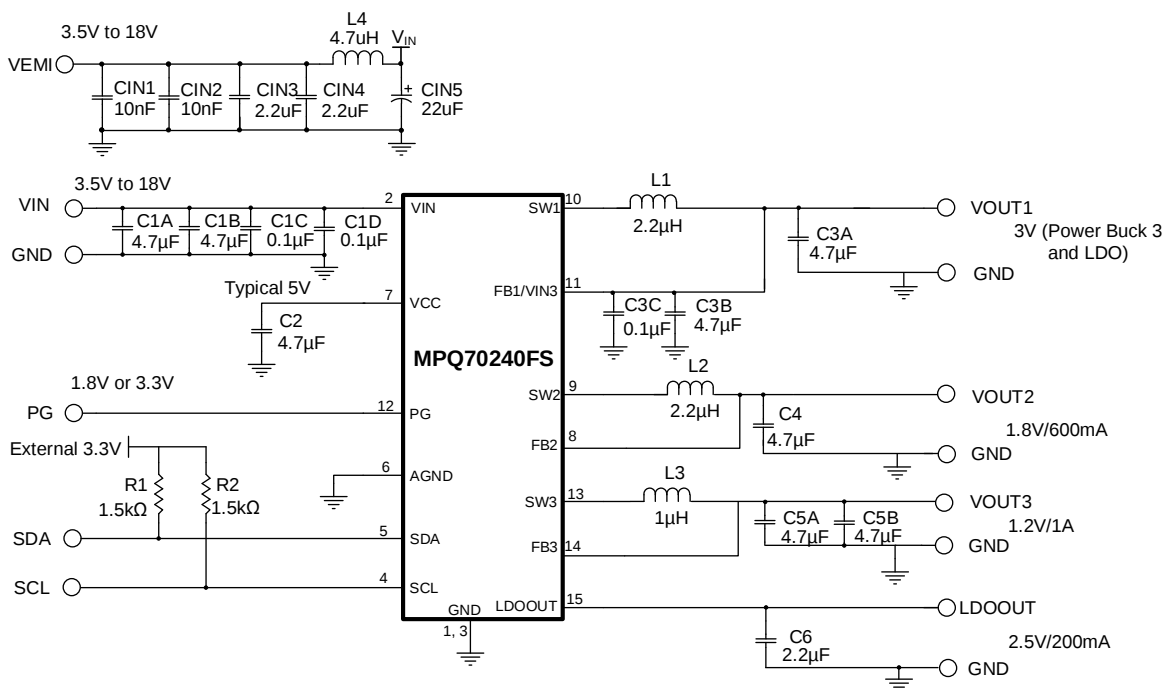
Figure 17: Typical Application Circuit with EMI Filters ( V_{OUT1} = 3V , V_{OUT2} = 1.8V , V_{OUT3} = 1.2V , V_{LDOOUT} = 2.5V )
