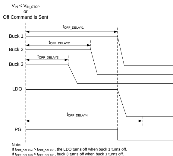
Figure 8: Shutdown Sequence
