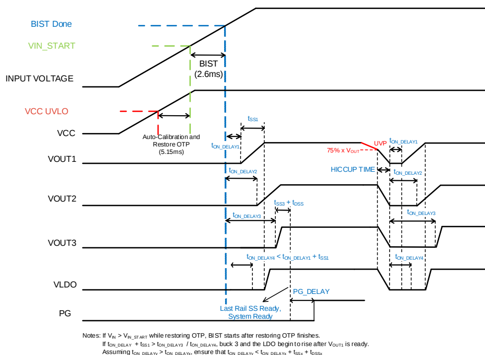
Figure 3: Power-On Sequence
