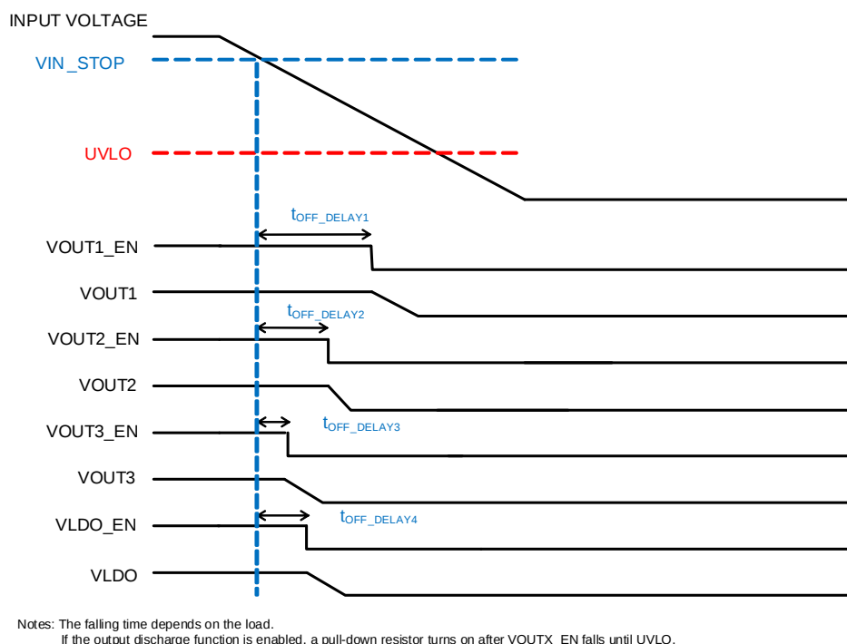
Figure 4: Power-Off Sequence
