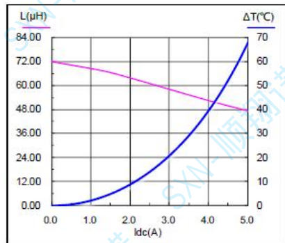
SMMS1350-680M
