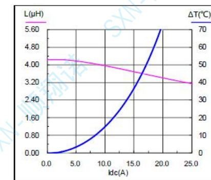
SMMS1350-4R7M
