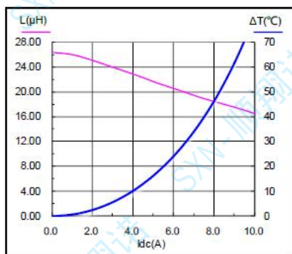
SMMS1350-680M
